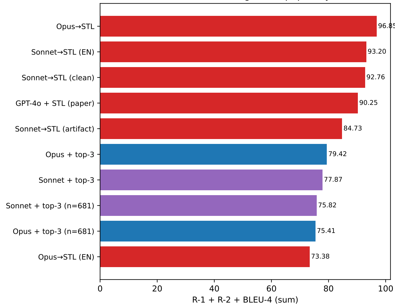
Surface-form ranking (KELE-paper-style)
