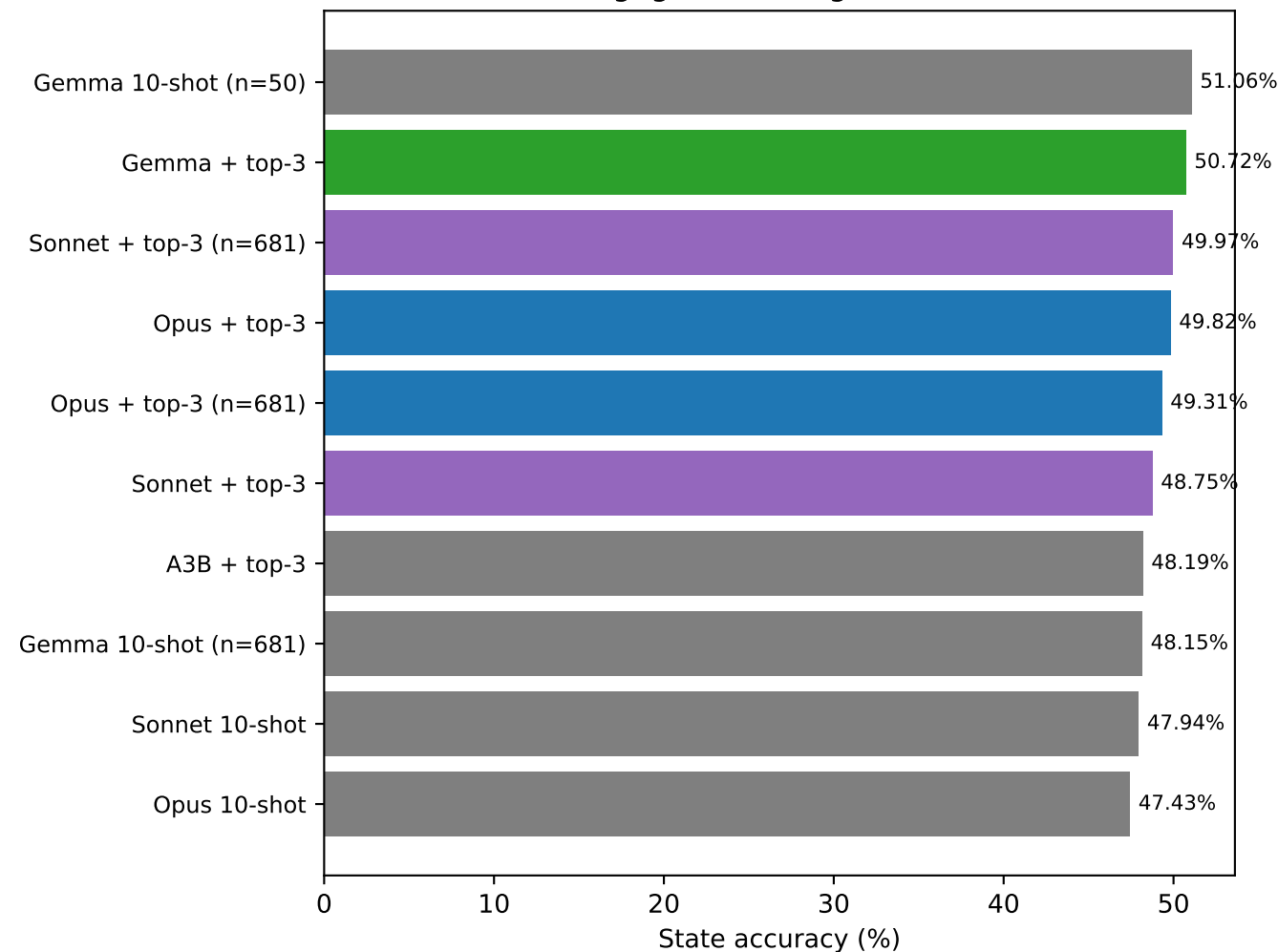
Pedagogical ranking (state acc)
