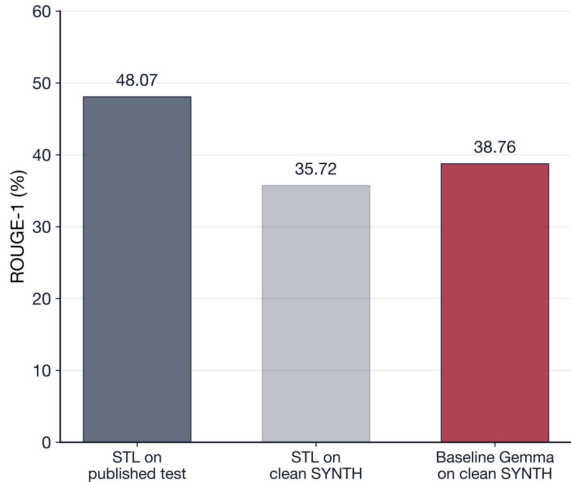
ROUGE-1 collapses with it
