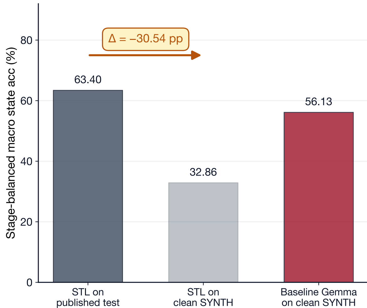
Stage routing collapses on unseen data
