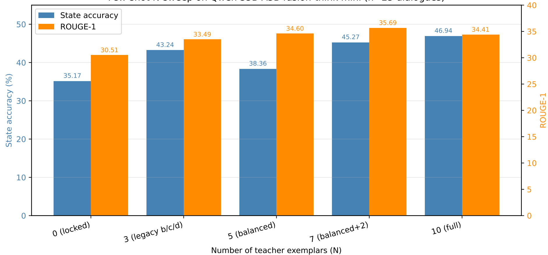
Few-shot N-sweep on Qwen 35B-A3B fusion-think mini (n=25 dialogues)
