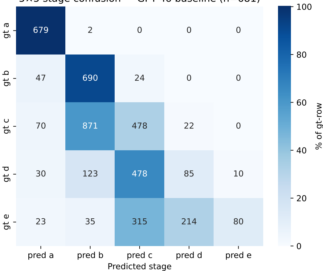
5×5 stage confusion — GPT-4o baseline (n=681)
