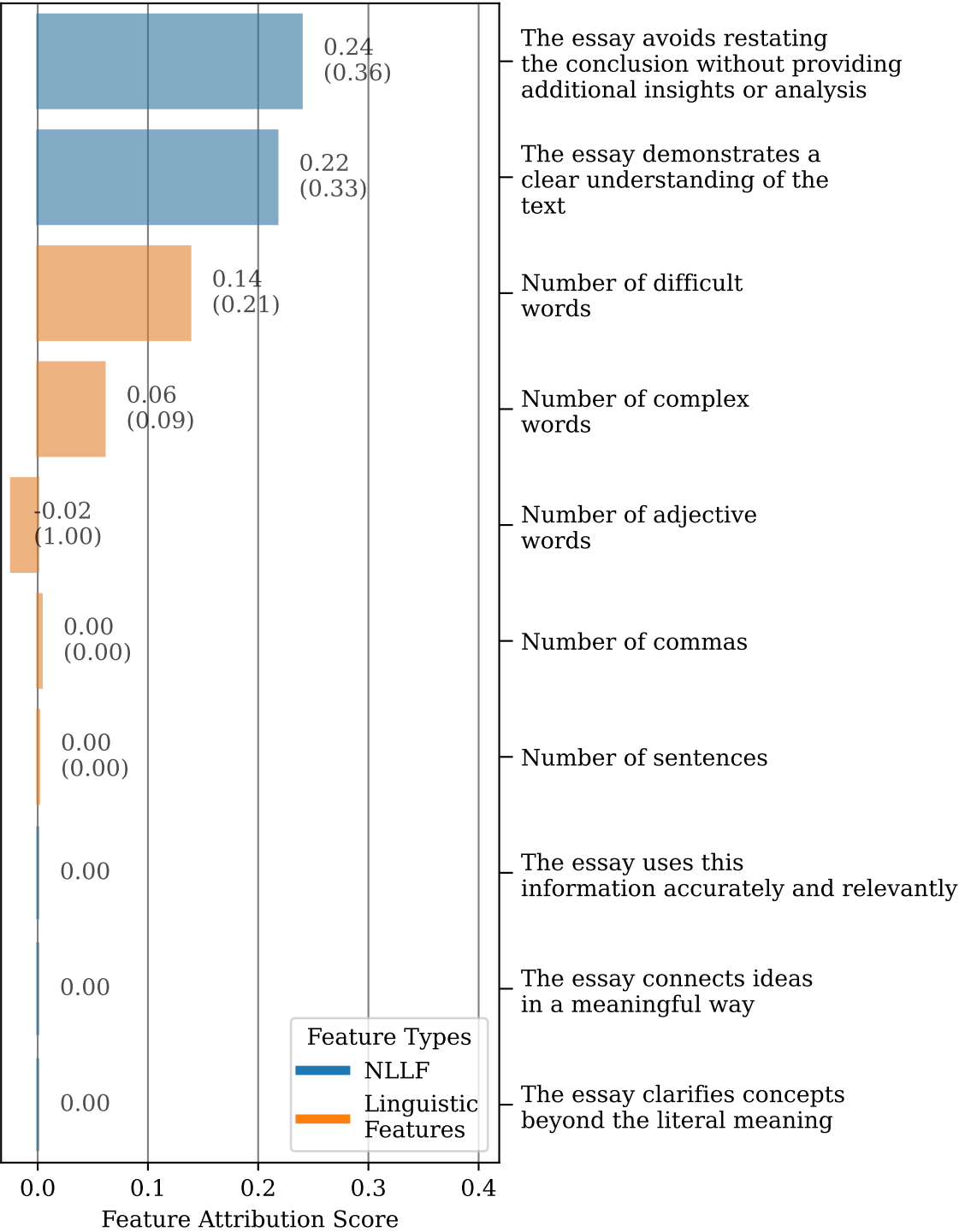
Top-10 Higher Feature Attribution Score
