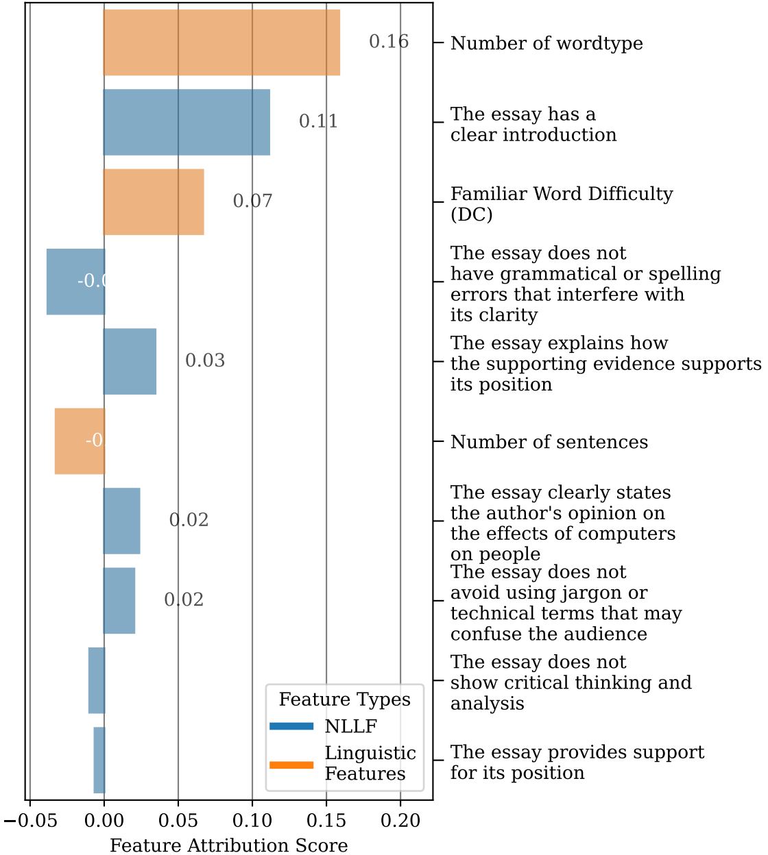
Top-10 Higher Feature Attribution Score
