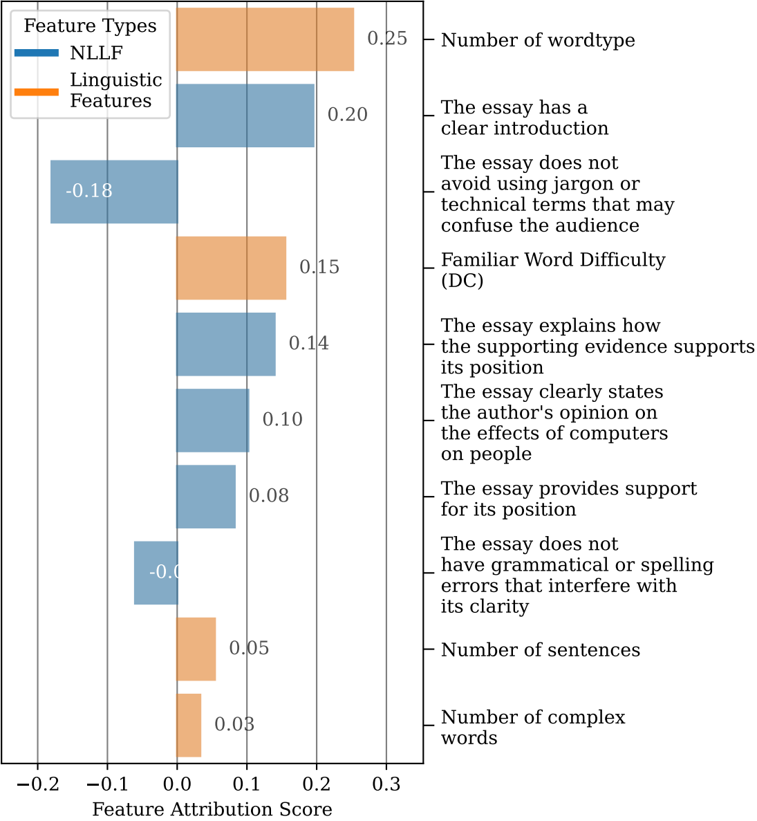
Top-10 Higher Feature Attribution Score
