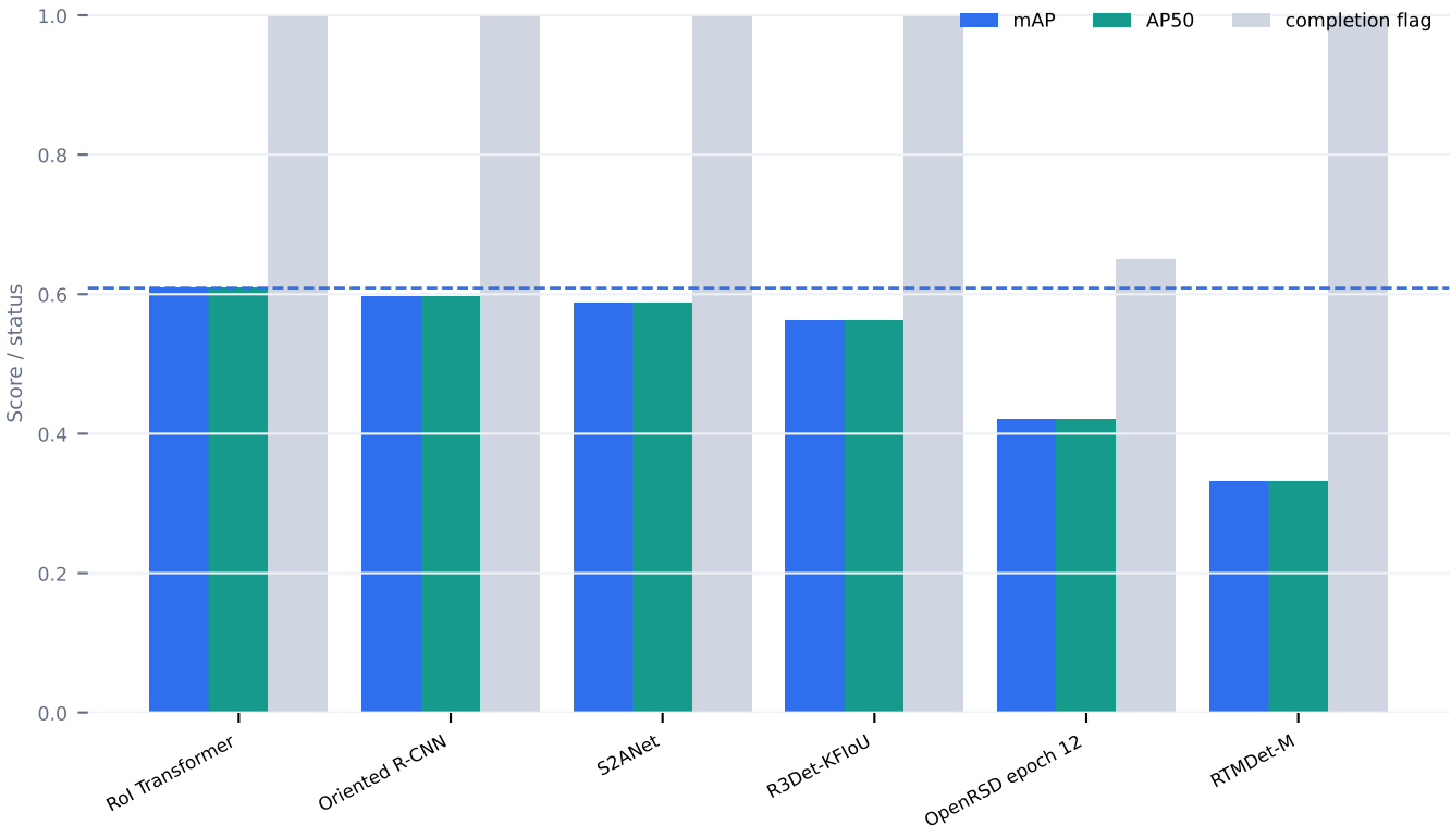
Detector-family score/status comparison
