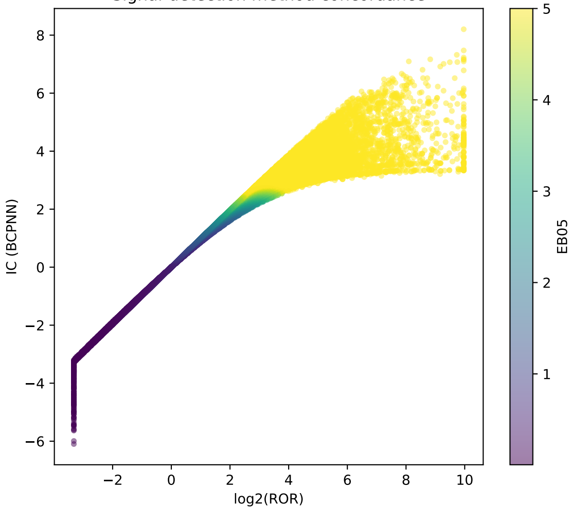
Signal-detection method concordance
