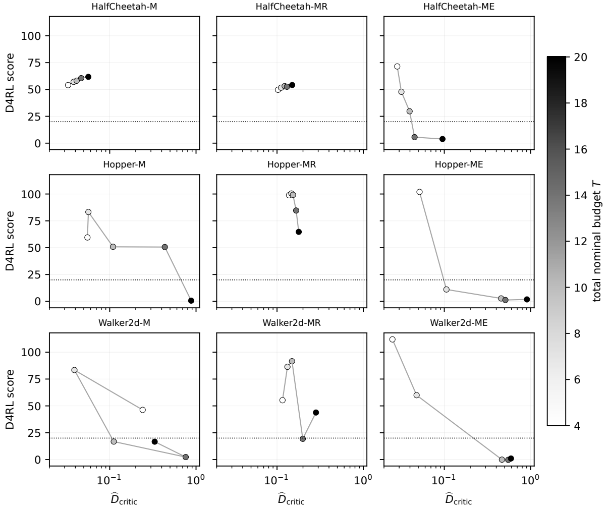
Figure 1: Environment-wise return versus the current-state \hat{D}_{\text{critic}} proxy for BAR-Prox K = 2 . Points are two-seed means for the common-batch audit at T \in \{4, 7, 10, 14, 20\} ; shade denotes T . Lines connect increasing T , exposing reversals rather than imposing a monotone response. Shared axes show that realized movement organizes several within-task transitions but does not define a universal cross-task failure threshold. The proxy does not measure the next-state Polyak target-policy movement.
