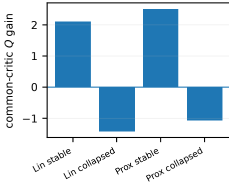
(c) Cross-critic validity
