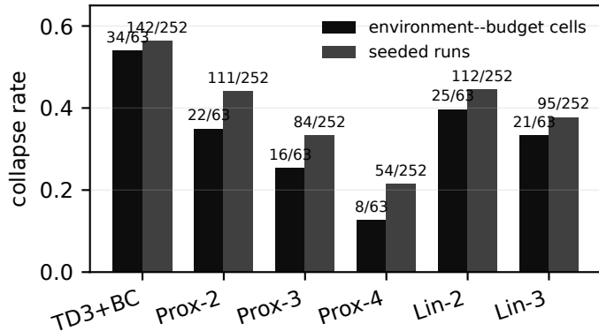
(b) High-budget collapse ( T \geq 4 )
