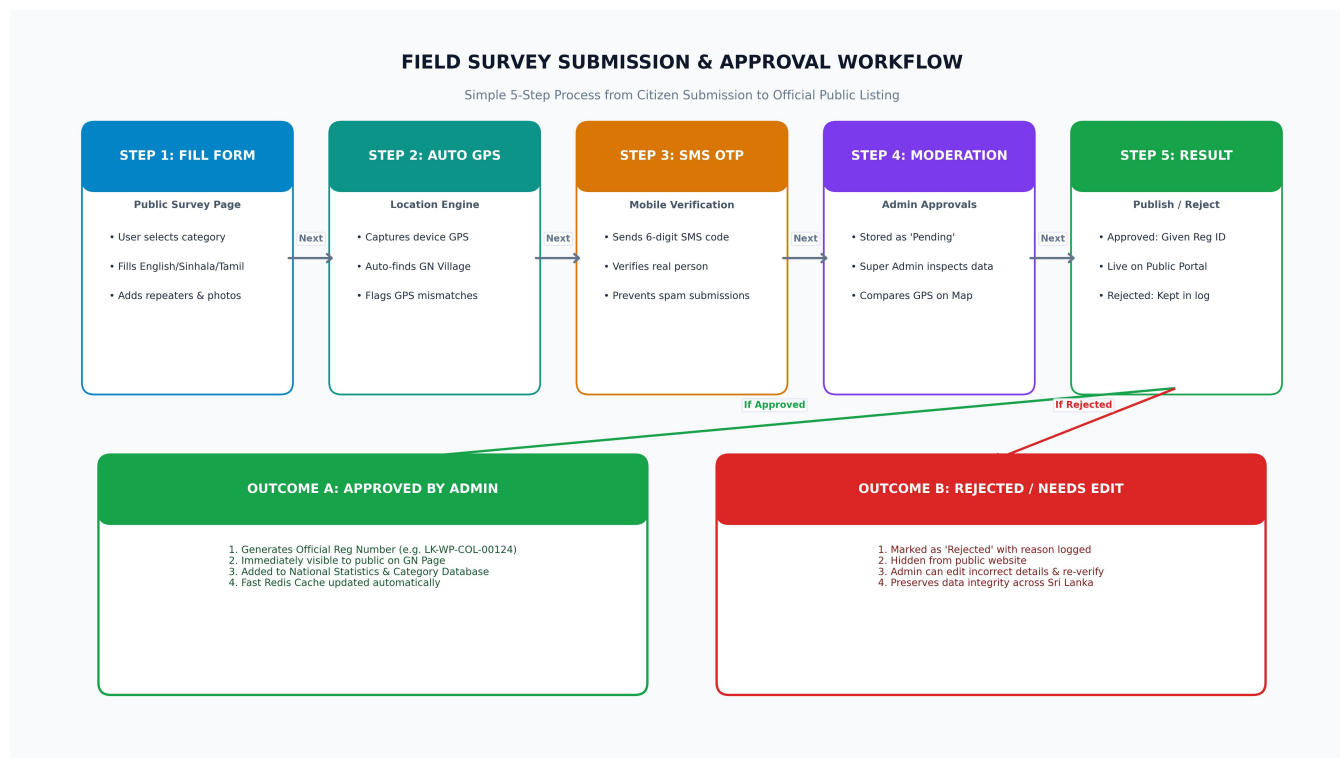
Figure 5.1: 5-Step Survey Submission & Approval Workflow
