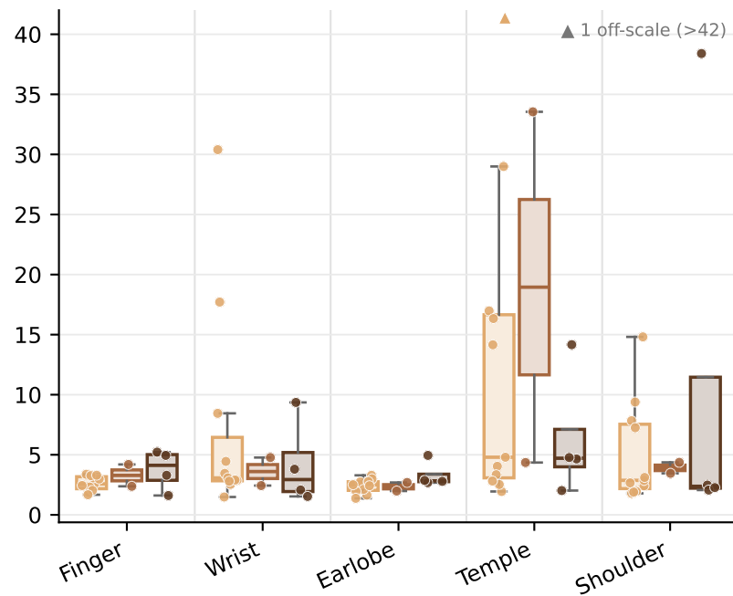
Kurtosis SQI (KSQI)
