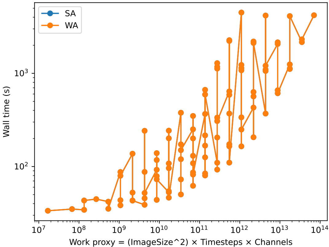
Wall-time scaling vs work proxy (log-log)
