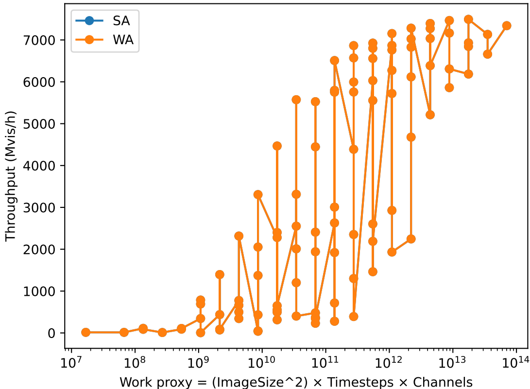
Throughput vs work proxy
