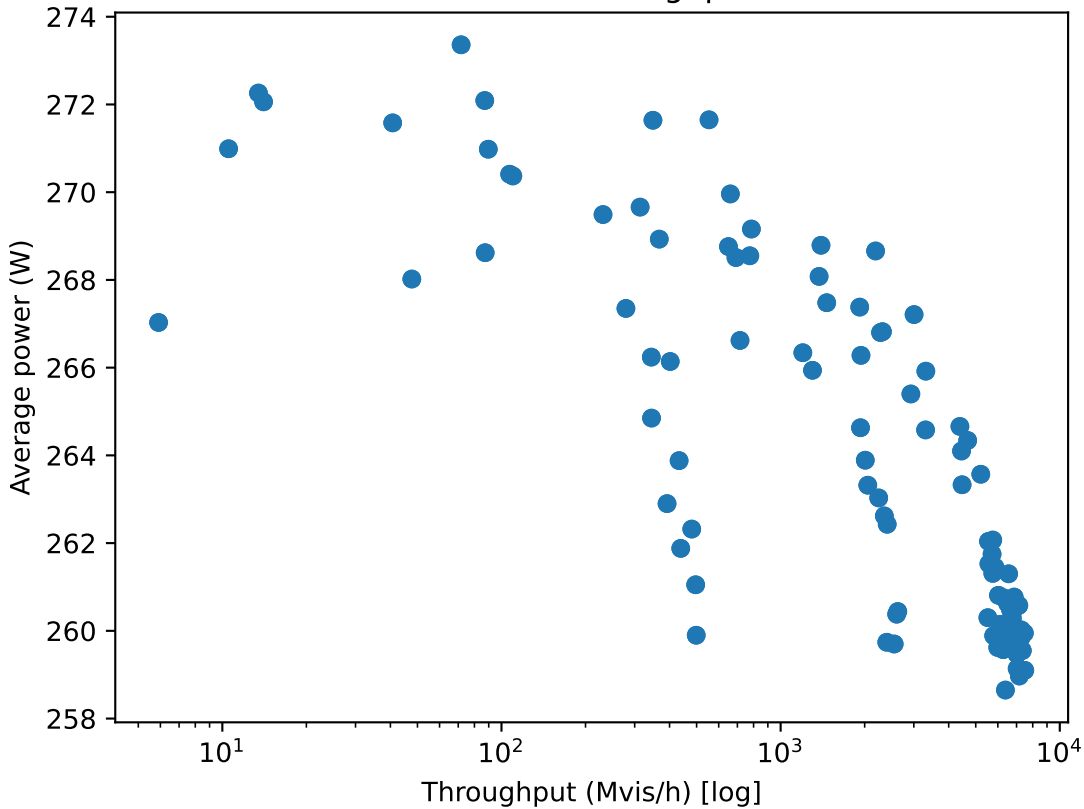
Power vs throughput
