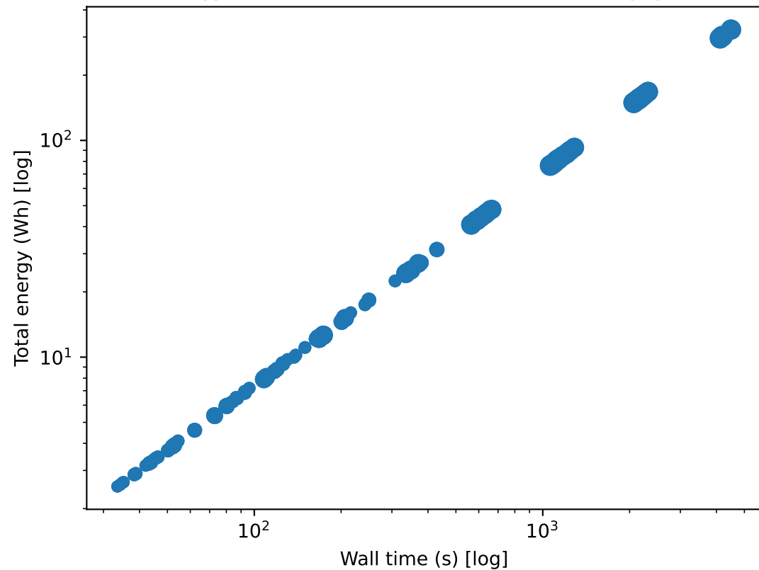
Energy-time tradeoff (marker size \propto throughput)
