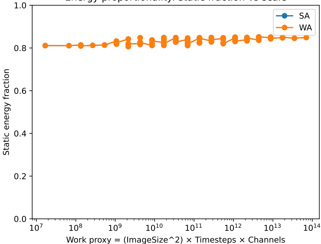
Energy proportionality: static fraction vs scale
