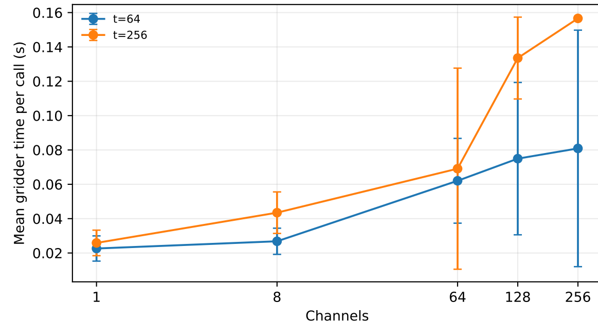
Per-call gridder duration and variability
