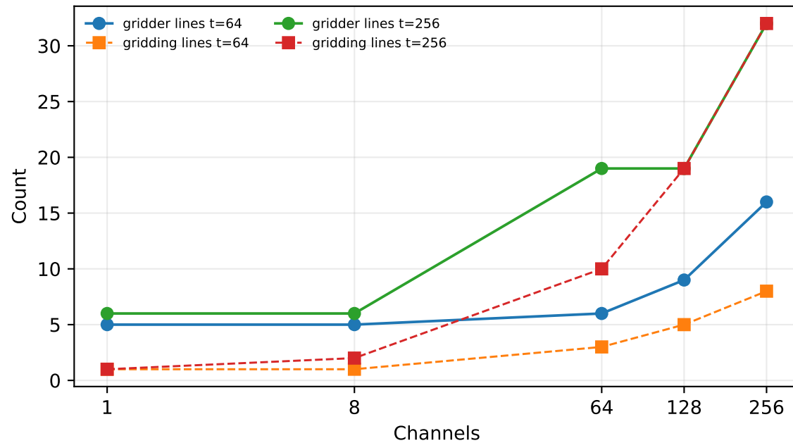
Parsed call counts from gridding and gridder lines
