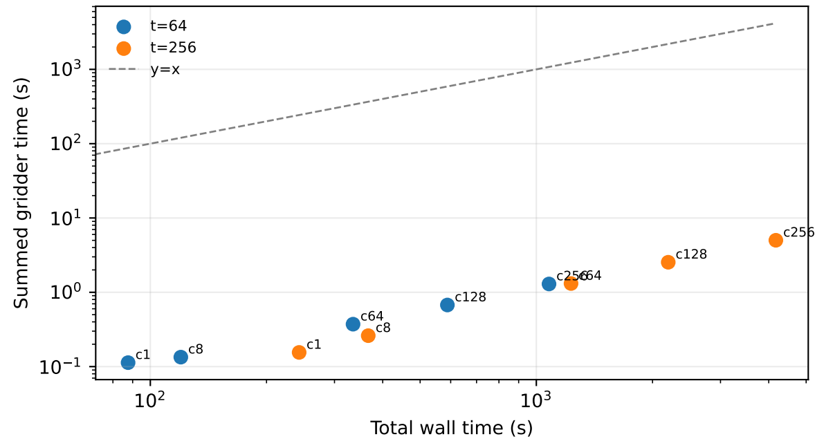
Summed gridder time tracks total wall time
