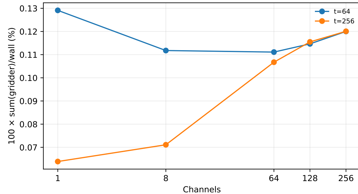
Gridder runtime share across channel scaling
