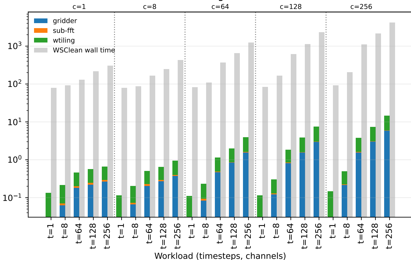
Kernel breakdown merged with total wall time
