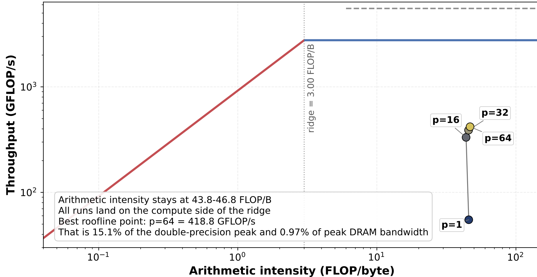
CPU Roofline
