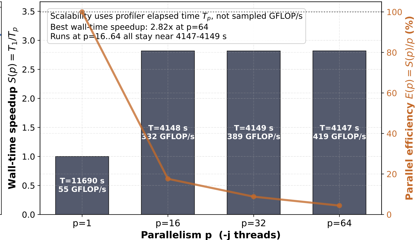
Scalability Summary
