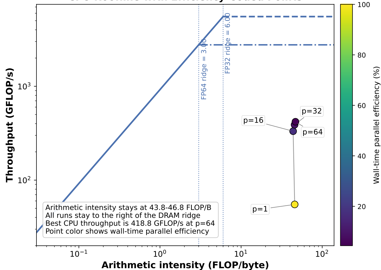
CPU Roofline with Efficiency-Coded Points
