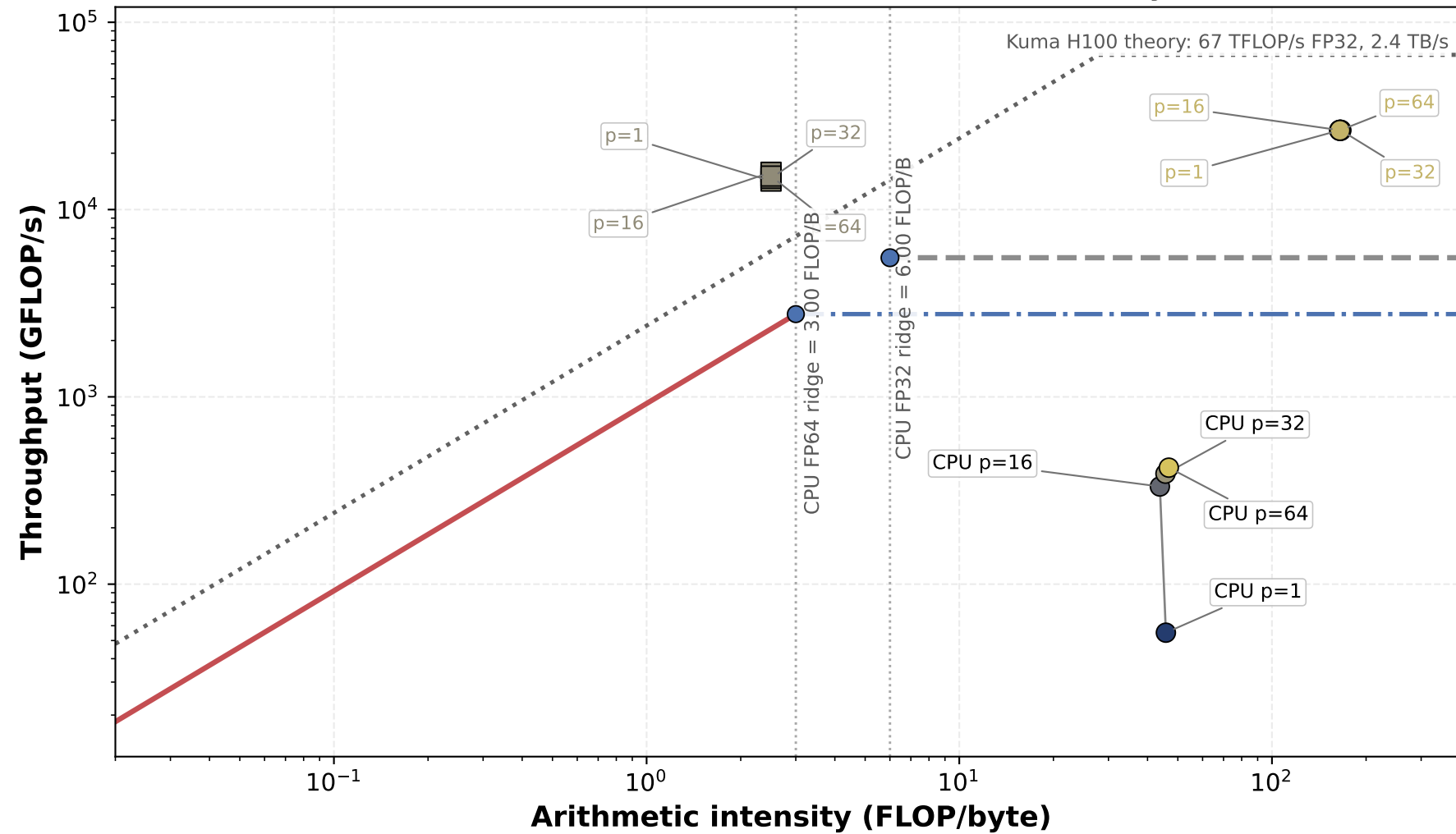
CPU Hardware Roofline vs GPU Kernel Roofline-Style View
