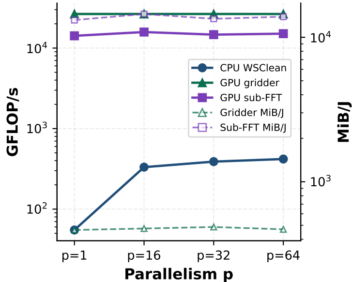
Matched-p Throughput and MiB/J
