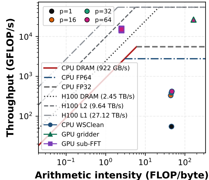
Roofline Comparison
