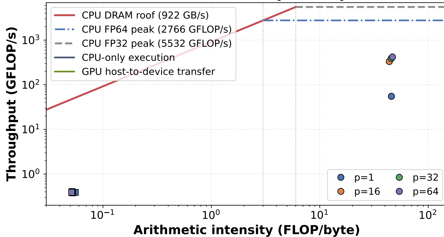
Roofline Summary Overlay
