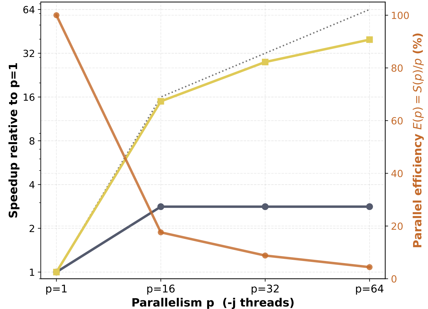
Gridding speedup outruns end-to-end speedup
