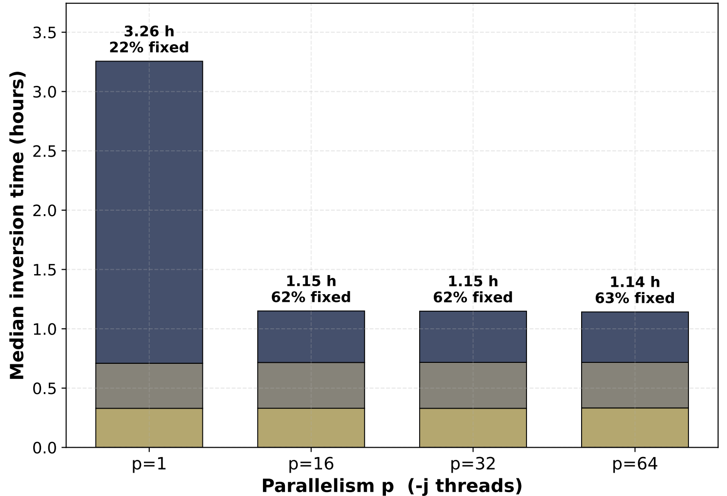
Median inversion-time decomposition
