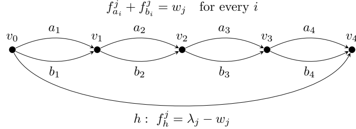
Figure 2: The flat chain G_4 . Each serial pair carries the same statewise branch flow w_j ; the bypass carries the remainder. All capacities and the source–sink flow value are one. Independent scalar totals at the four pairs do not retain the common vector of state flows. The general G_L extends the same pattern to L pairs.
