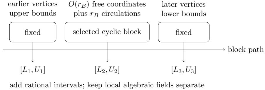
Figure 2: Nomination localization for a terminal difference. Independent coefficients may still be optimized in every block; “fixed” refers to aggregated nominations. The selected block is cyclic; bridge cases are handled directly. The number of blocks is unrestricted.
