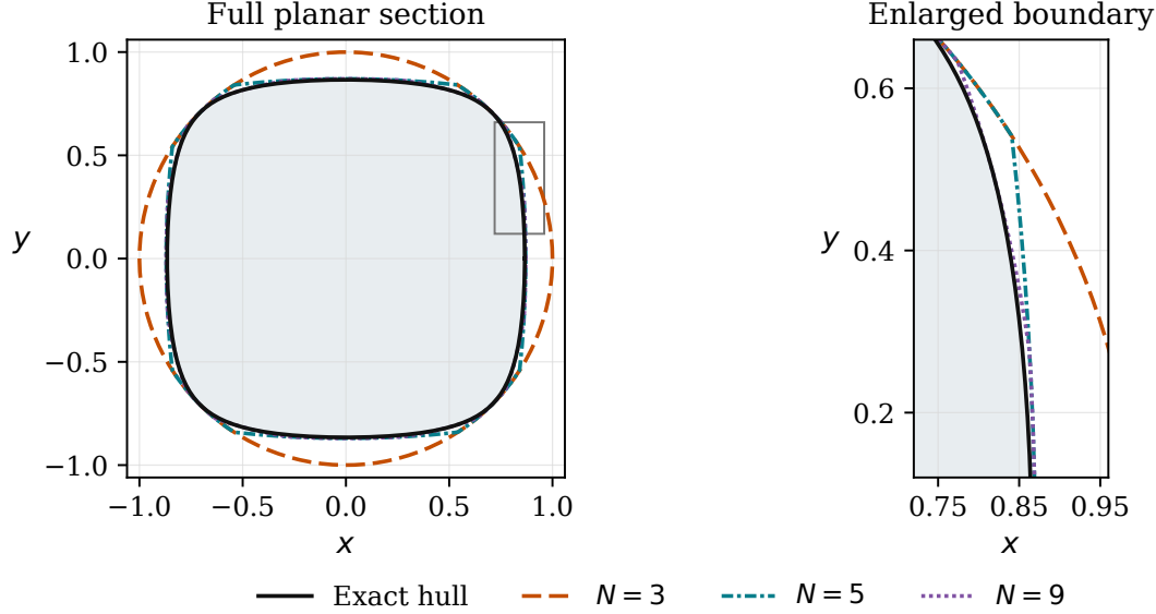
Figure 1: Sections by the plane u = xe_1 , v = ye_2 . The exact closed hull (black) is (1 - x^2)(1 - y^2) \geq 1/4 inside the unit square bounds. Colored curves bound the outer approximations from N = 3, 5, 9 equally spaced angles in Lemma 7.2; the right panel enlarges part of the first quadrant. The same planar sections occur for every r \geq 2 . The curves are computed from explicit radial formulas and illustrate the approximations; they are not estimates of their full Hausdorff errors.
