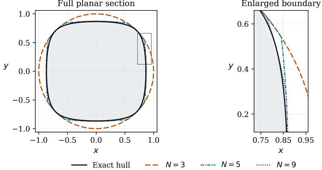
Figure 1: Sections by the plane u = xe_1, v = ye_2 . The exact closed hull (black) is (1 - x^2)(1 - y^2) \geq 1/4 inside [-1, 1]^2 . Colored curves bound the outer approximations from N = 3, 5, 9 equally spaced angles in Lemma 8.2; the right panel enlarges part of the first quadrant. The same planar sections occur for every r \geq 2 . The curves are computed from explicit radial formulas and illustrate the approximations; they are not estimates of their full Hausdorff errors.
