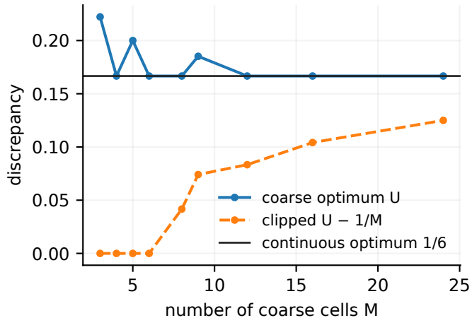
Uniform input: n = 3 , s = 2 , T = 1
