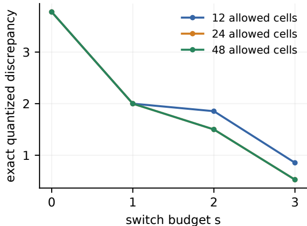
Public profile, T = 12
