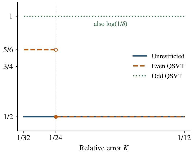
(b) Proved parity separation, \rho = 2
