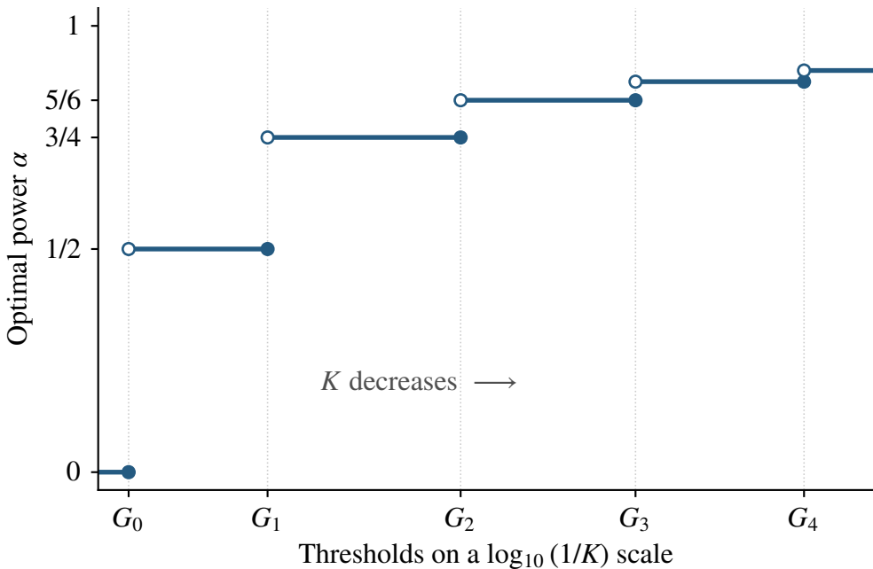
(a) Unrestricted conversion, \rho = 2
