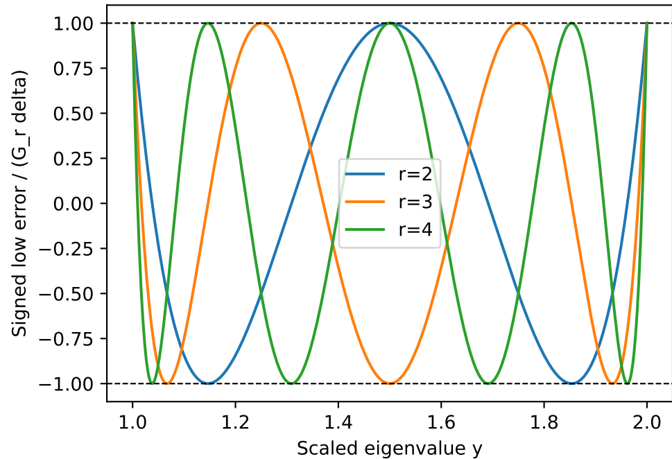
Pinned threshold errors (diagnostic)
