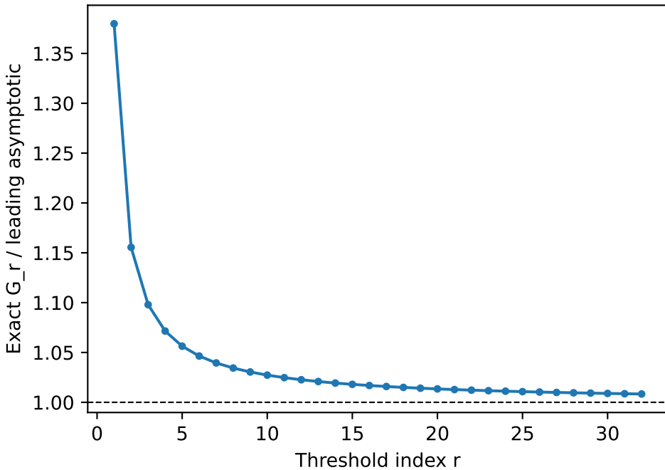
Threshold asymptotic, \rho = 2
