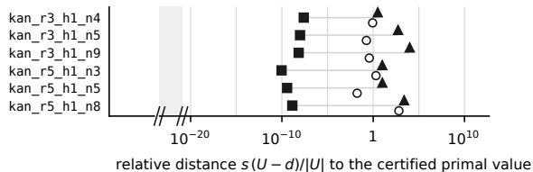
(b) KAN instances. Different models: certified lower bound for \mathcal{R} ; listed and one-hour bounds for the stored models (descriptive)
