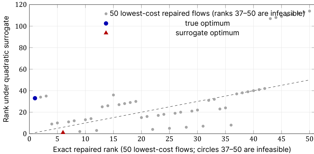
Figure 1. Surrogate rank audit for the 50 lowest-cost repaired flows. Exact enumeration confirms there are exactly 36 feasible flows (ranks 1–36); the remaining 14 shown here are infeasible flows at higher repaired energies. The surrogate has high global R^2 but imperfect low-energy ordering: the exact optimum is only rank 33 under the surrogate, while the surrogate minimum repairs to the sixth-best exact flow. Quantum-sampling outcomes are therefore scored using the exact repaired objective F , not the surrogate \hat{F} .
