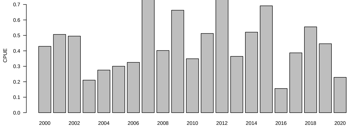
Average CPUE of tournament-caught dolphinfish by year
