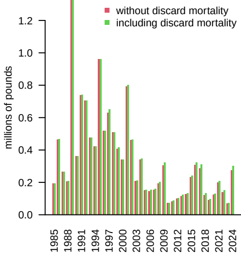
Hire_NCFL
