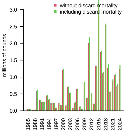
Rec_VBM
