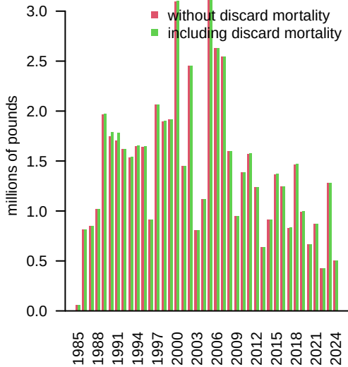
Hire_VBM
