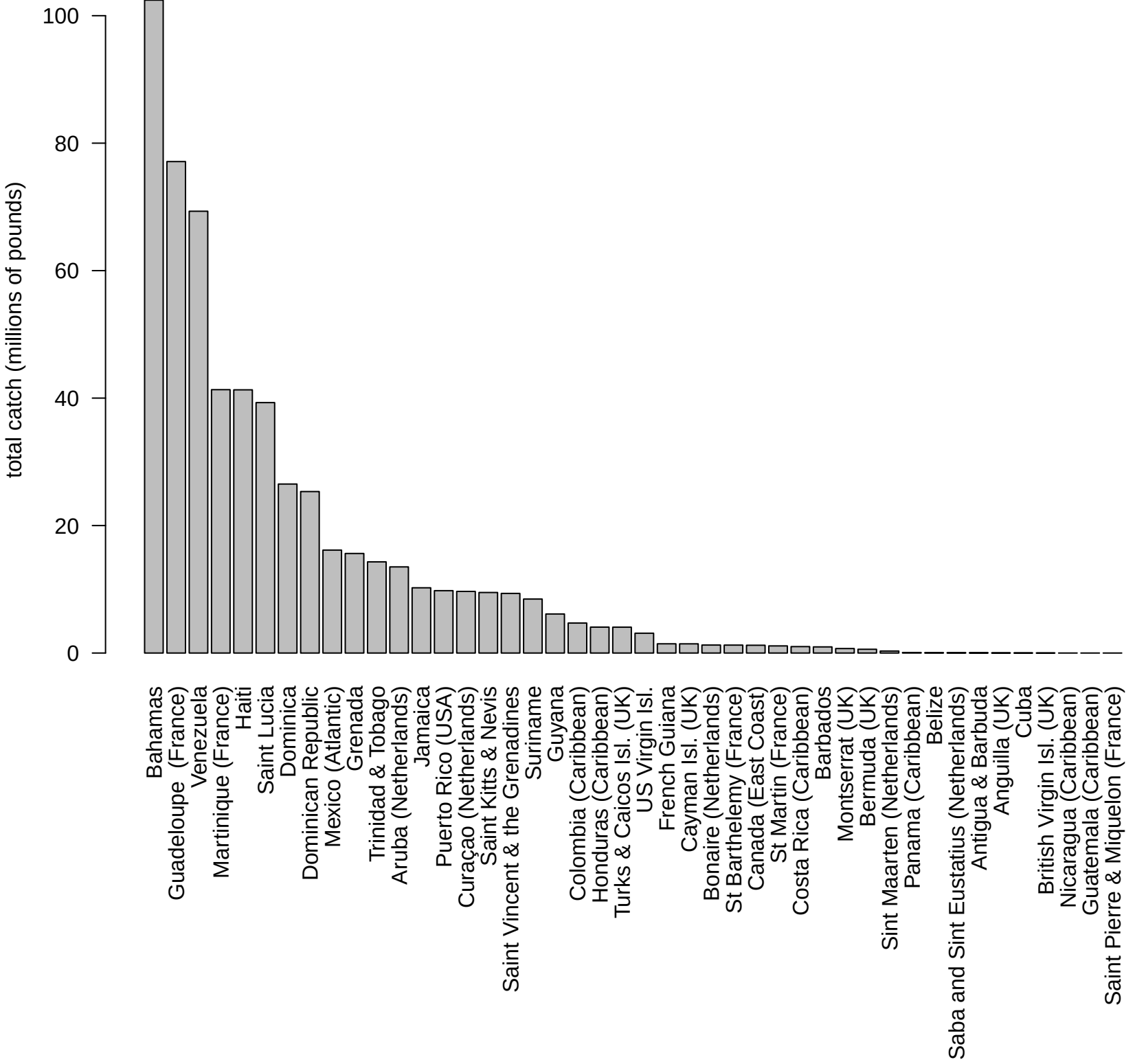
Total dolphin catch (1950 – 2022) in the Western Atlantic, by EEZ
