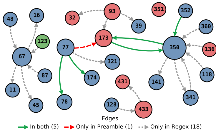
(a) Preamble vs. Regex
