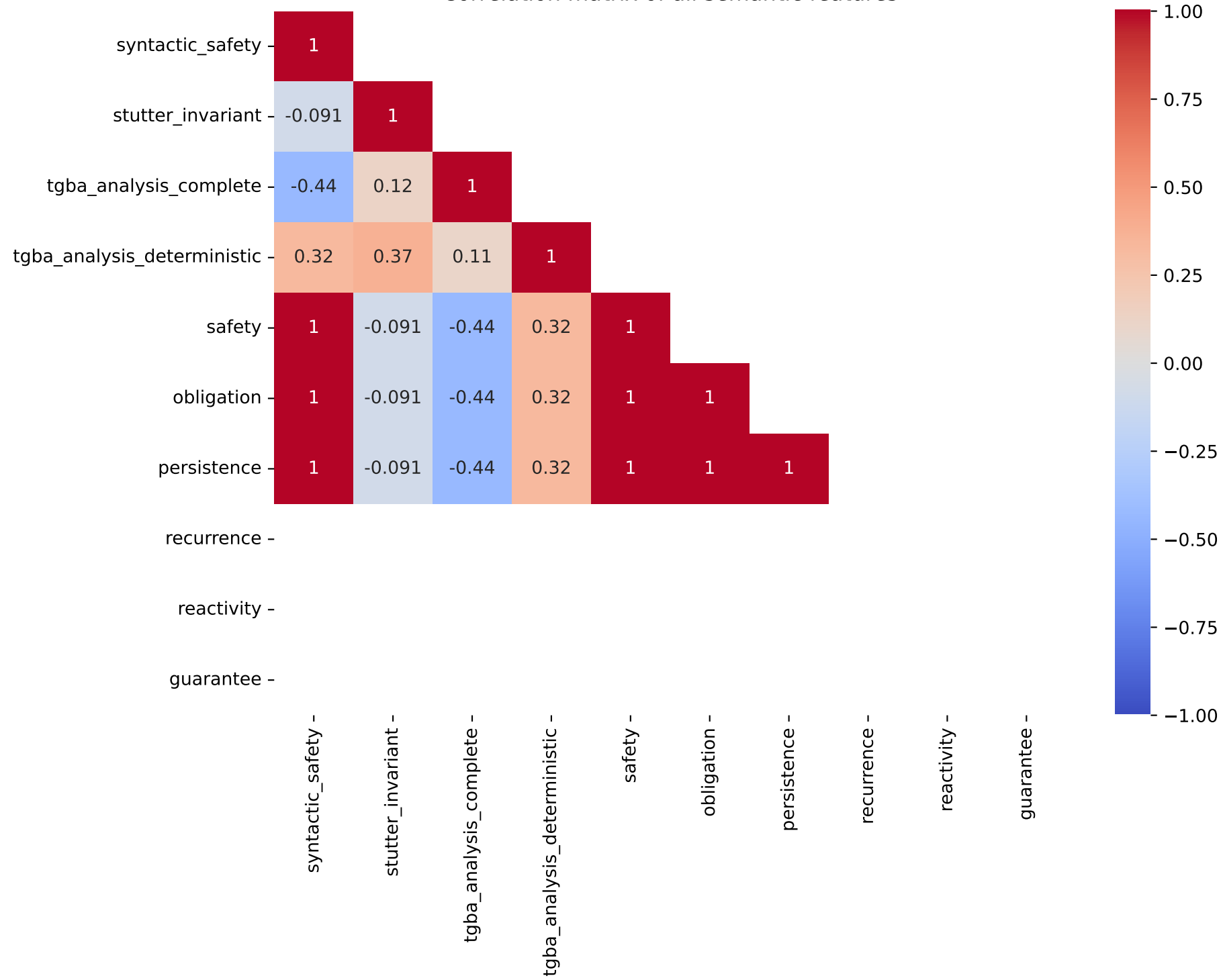
Correlation matrix of all semantic features
