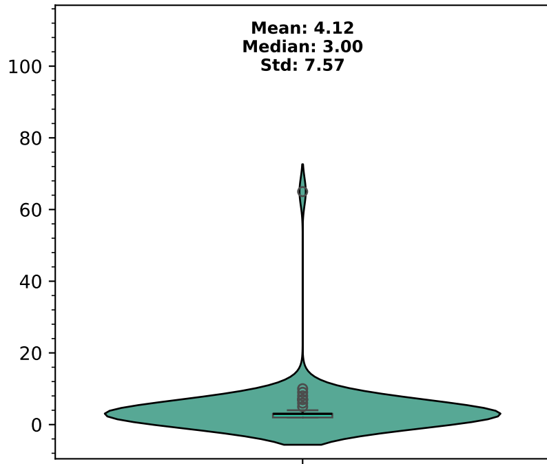
states_count
