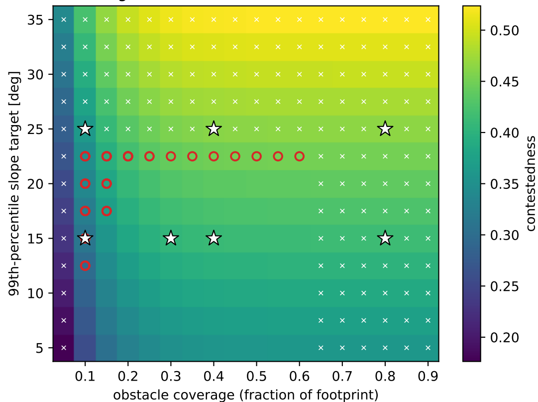
DOE grid at friction 0.6/0.5, restitution 0.1
