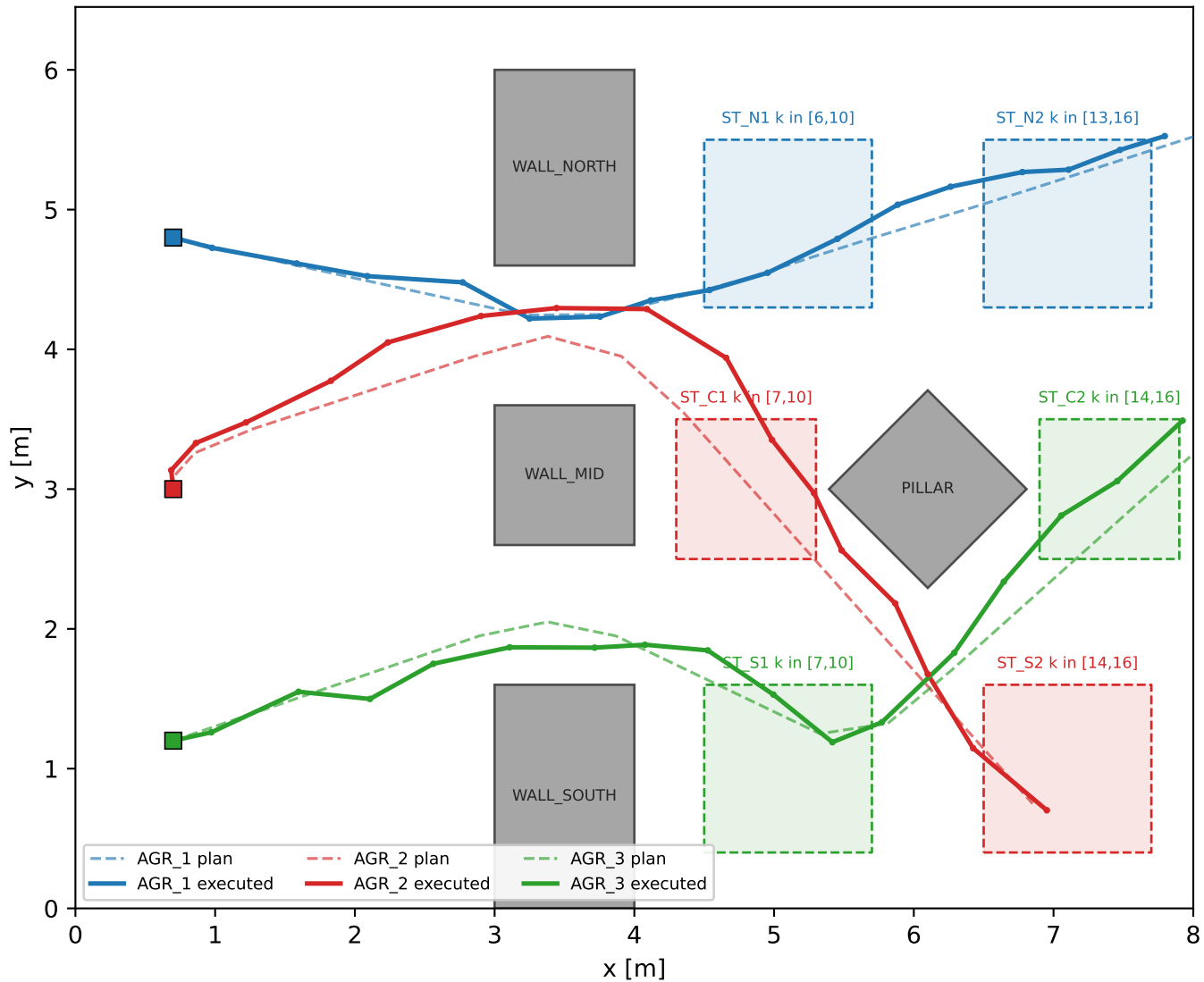
MILP plans (dashed) and executed trajectories (solid), seed 0
