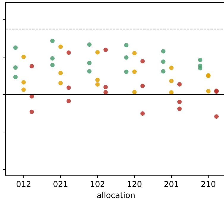
Executed robustness of every trial (dashed: the margin the plan holds); margin 0.5 m infeasible for every allocation required margin 0.15 m required margin 0.35 m required margin 0.45 m
