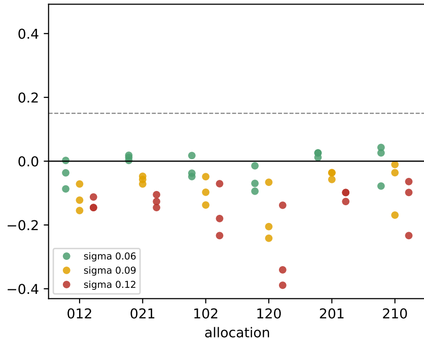
Executed robustness of every trial (dashed: the margin the plan holds); margin 0.5 m infeasible for every allocation required margin 0.15 m required margin 0.35 m required margin 0.45 m
