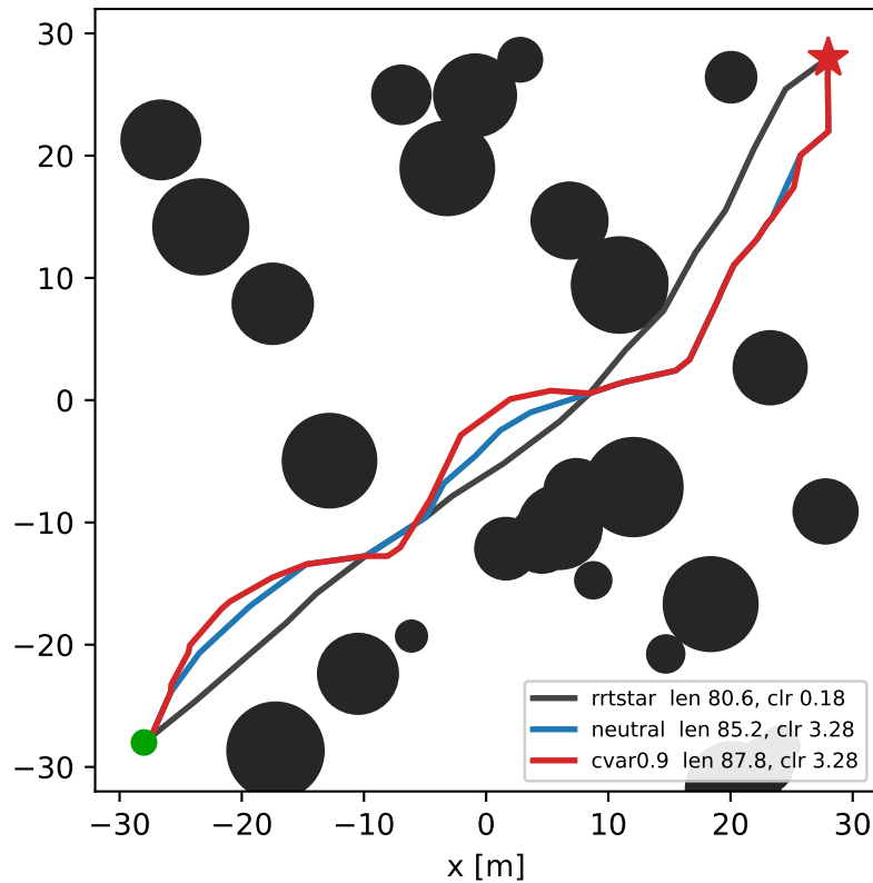
medium environment
