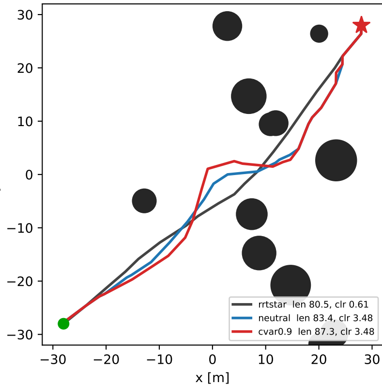
easy environment
