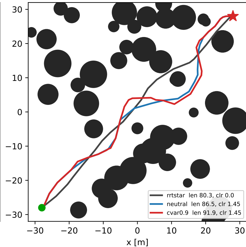
hard environment
