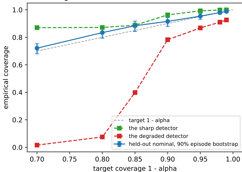
coverage on detections the calibration never saw
