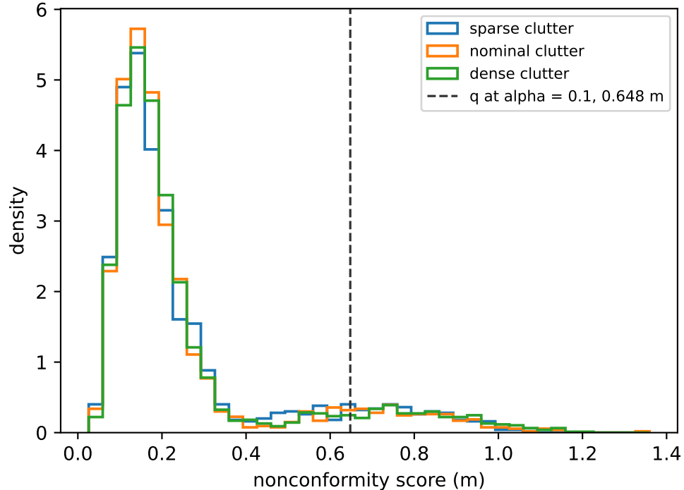
calibration scores of the nominal detector
