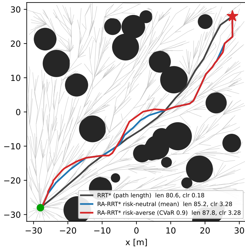
RRT* tree and planned paths, noise level 0.5
