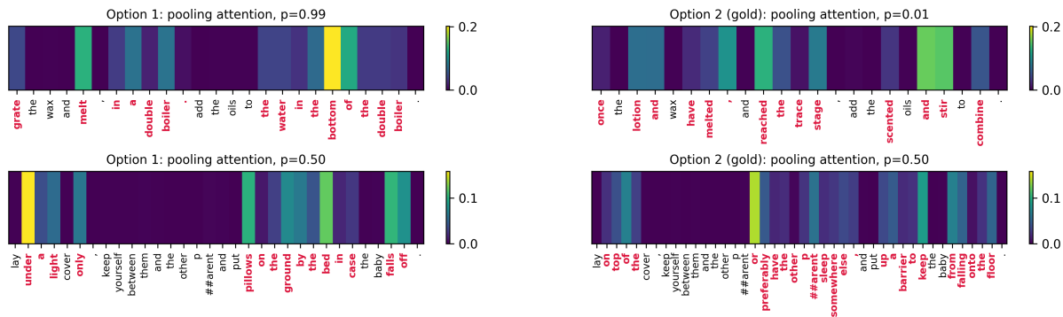
Figure 3: Pooling attention (bright = high; red = differing tokens). Top: adding scents to lotion bars , a confident error ( p = 0.99 for option 1). Bottom: to safely sleep with your baby in your bed , the most uncertain item ( p = 0.50 ; option 2 is gold).
