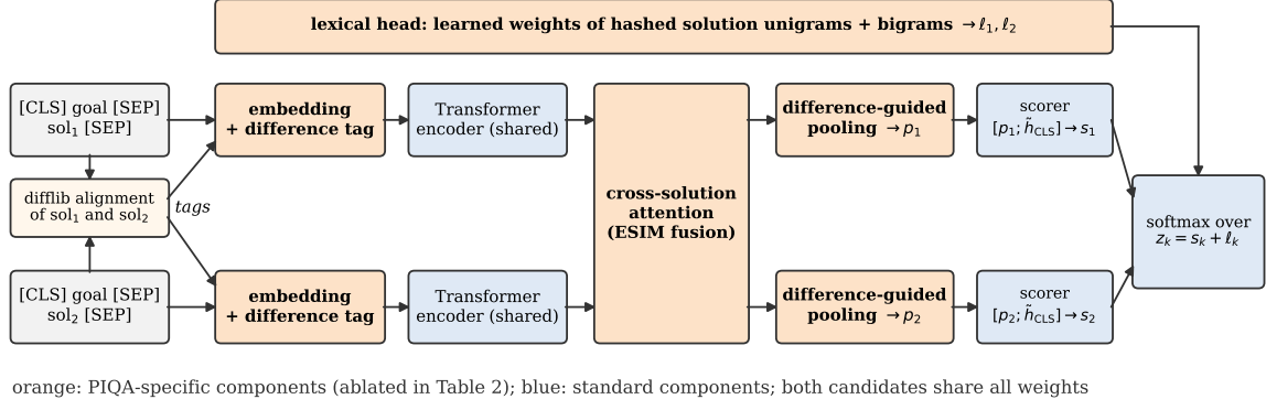
Figure 1: Architecture of DACT. The two candidates share all weights, so swapping two already-encoded candidates swaps their scores. The difflib alignment that produces the tags does depend on the order of the options (Section 4.5).
