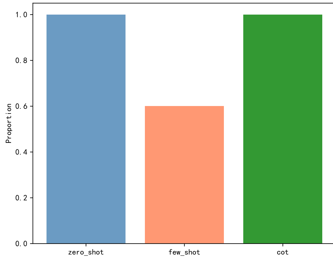
Code Block Inclusion Rate
