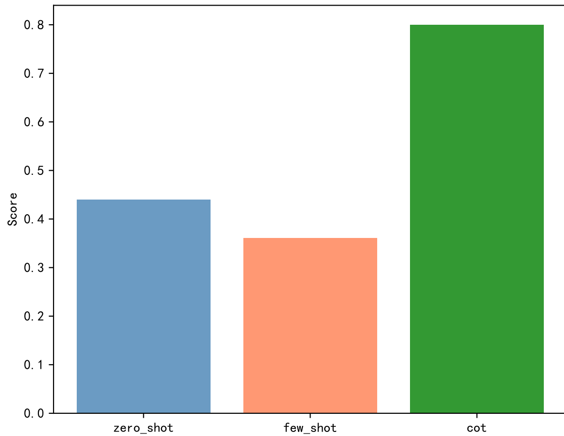
Completeness Score
