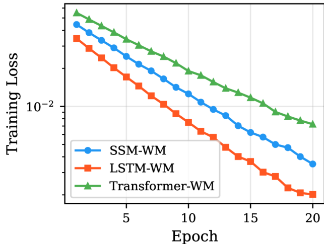
(a) Training Loss
