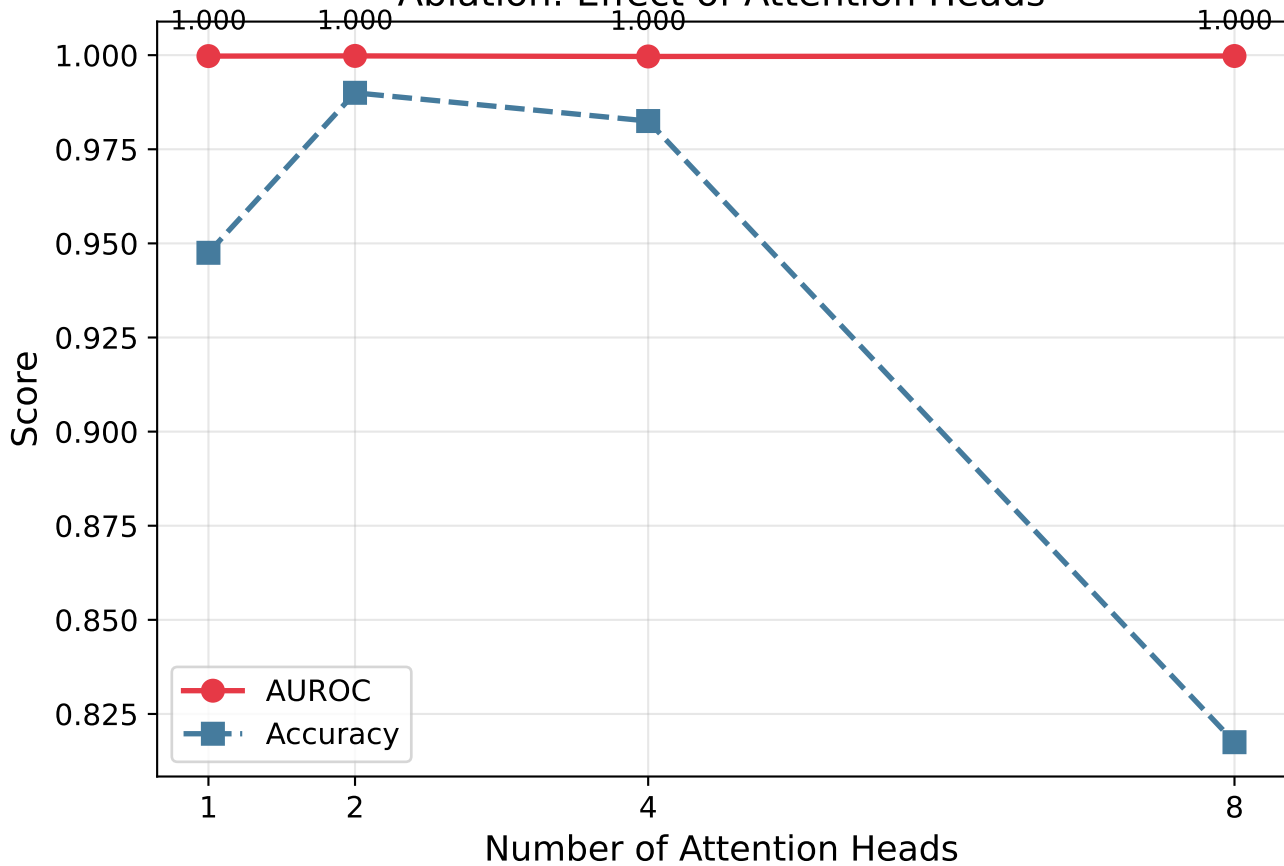
Ablation: Effect of Attention Heads
