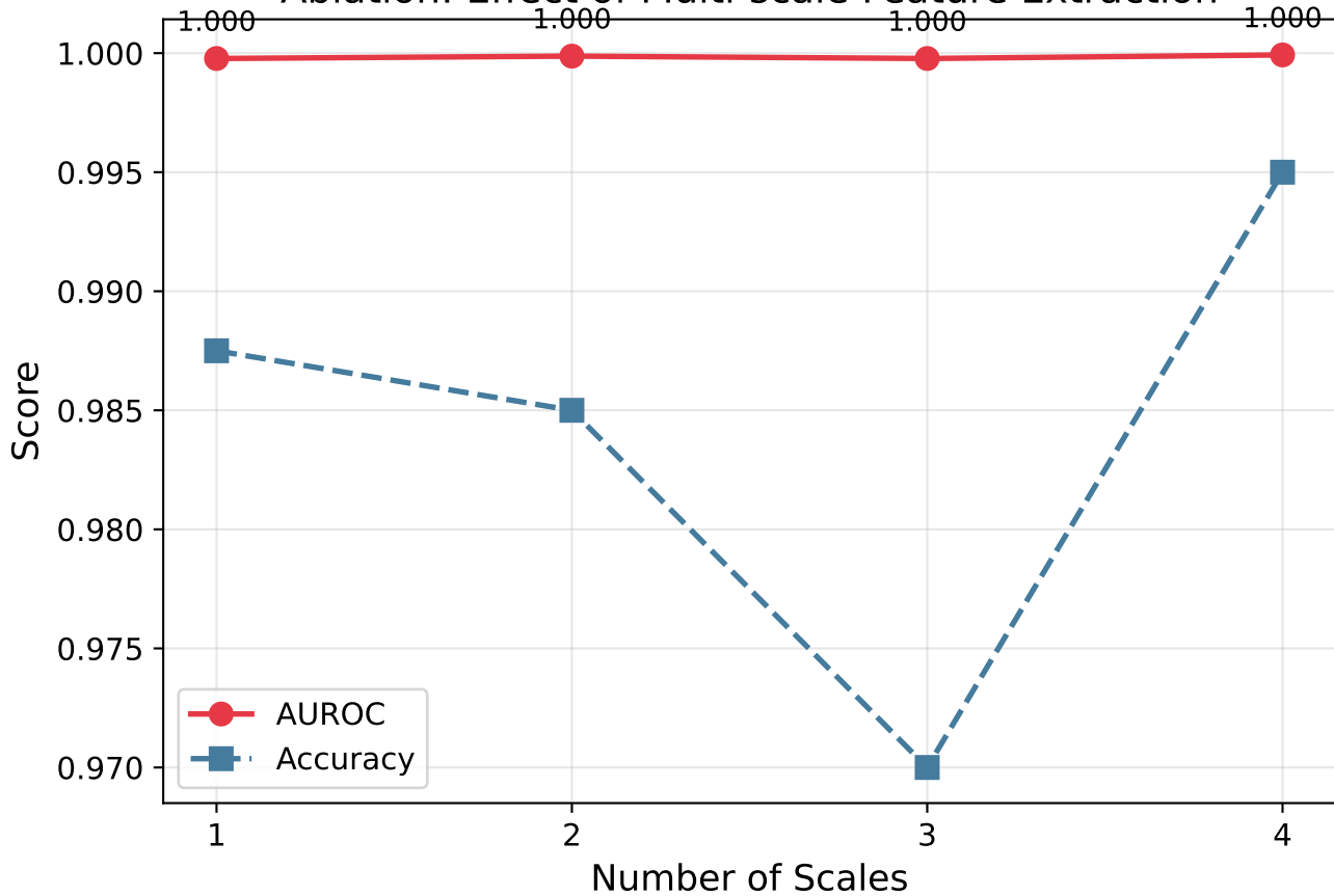
Ablation: Effect of Multi-scale Feature Extraction
